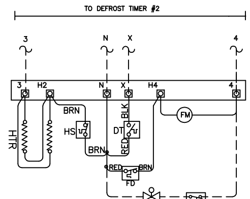
(B) DEFROST WIRING DETAIL SINGLE EVAP 208-230/60/1- V
