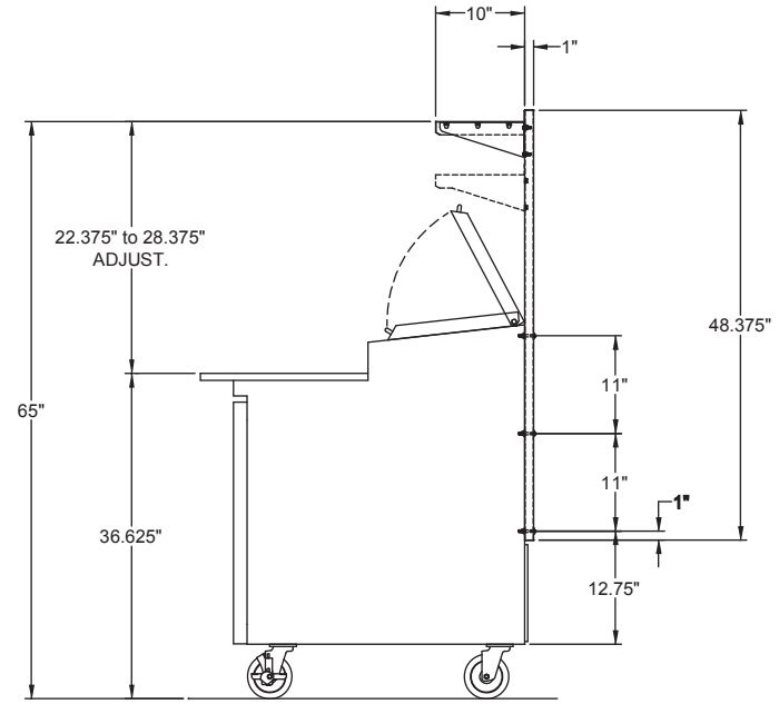
SECTION - 1
