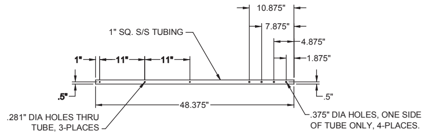
DETAIL, UPRIGHT
