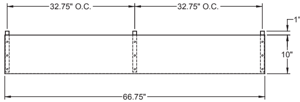
PLAN VIEW MBPT67 Pizza Prep
