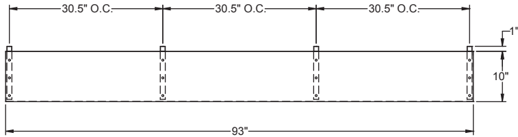
PLAN VIEW MBPT93 Pizza Prep
