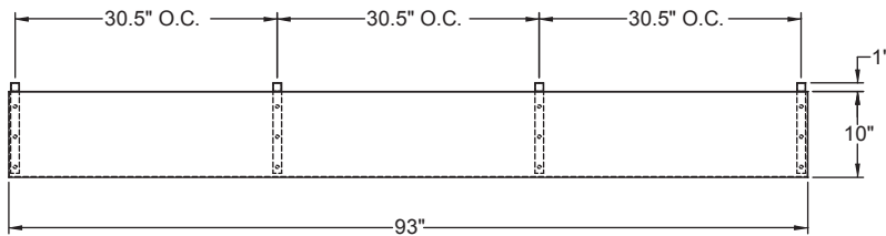
PLAN VIEW MBPT93 Pizza Prep
