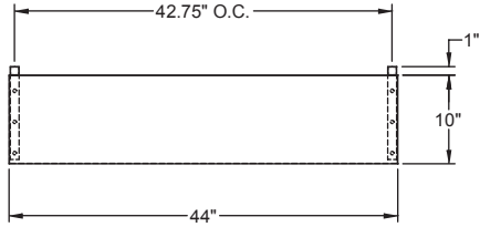
PLAN VIEW MBPT44 Pizza Prep
