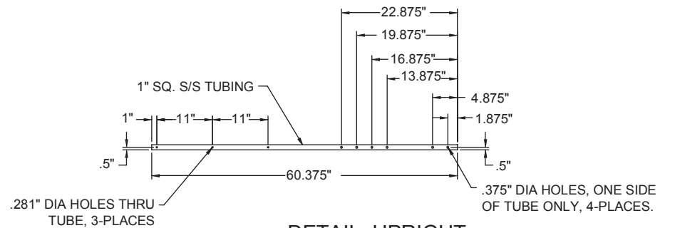
DETAIL, UPRIGHT
