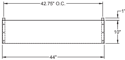
PLAN VIEW MBPT44 Pizza Prep
